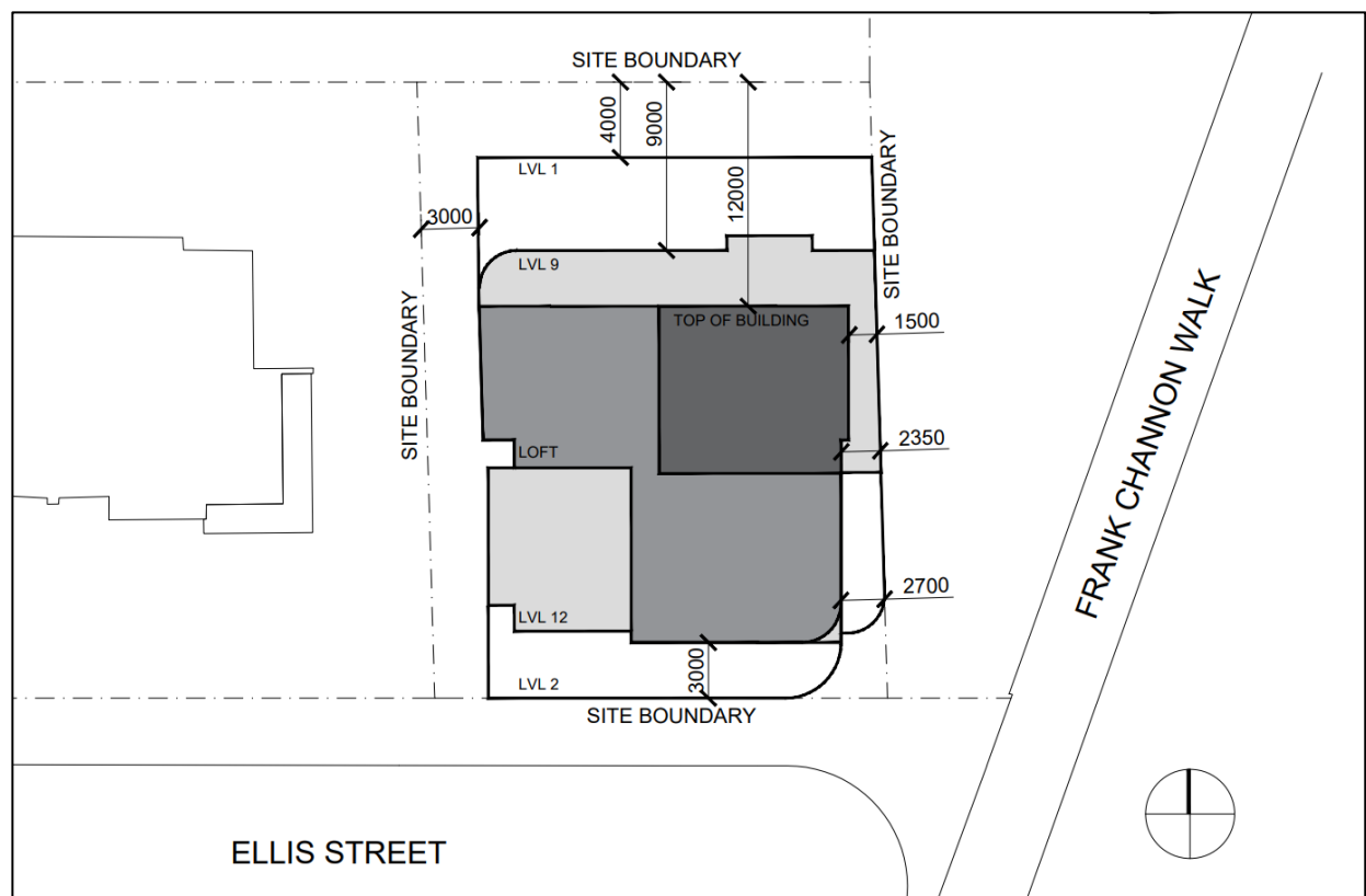
Figure 2: Building Setback
