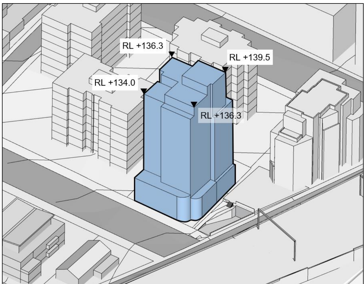
Figure 3: Building Height
